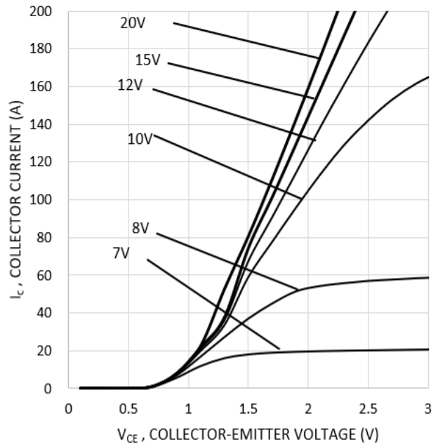
Fig. 2 Typical output characteristic (T vj =25°C)
