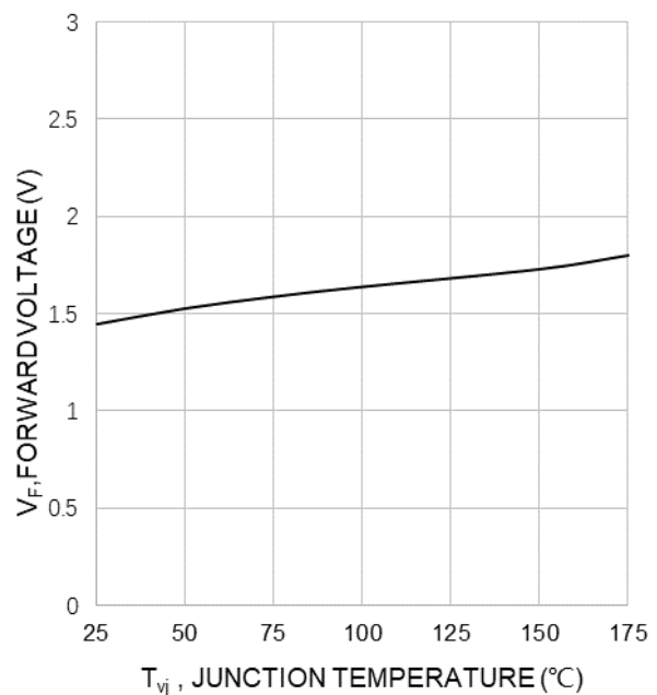
Fig. 12 Typical diode forward voltage as a function of junction temperature
