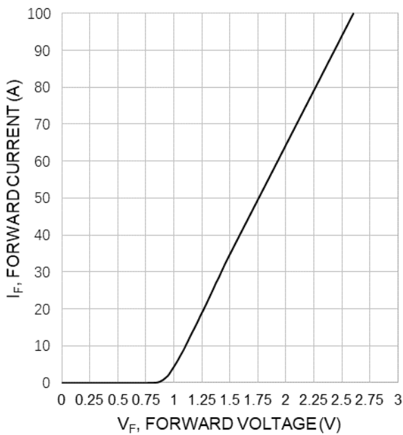
Fig. 11 Typical diode forward current as a function of forward voltage
