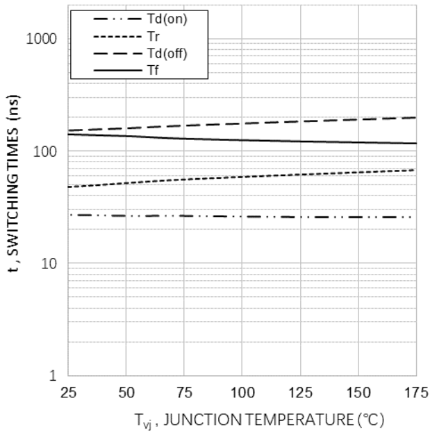
Fig. 9 Typical switching times as a function of junction temperature (inductive load, V CE =400V, V GE =15/0V, I C =37.5A, r G =8Ω)
