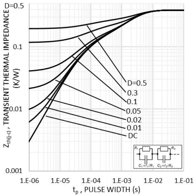
Fig. 15 IGBT transient thermal impedance ( D=t_p/T )
