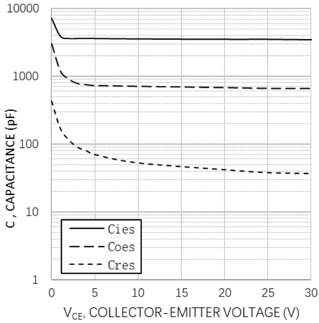
Fig. 13 Typical capacitance as a function of collector-emitter voltage ( V_{GE}=0V , f=1MHz )
