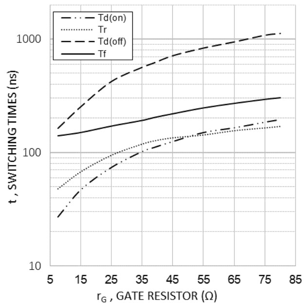
Fig. 8 Typical switching times as a function of gate resistance (inductive load, T_{yj}=25^{\circ}C , V_{CE}=400V , V_{GE}=15/0V , I_C=37.5A )
