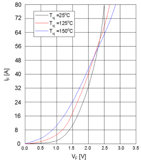
Fig. 4 Forward characteristic of Diode-Inverter
