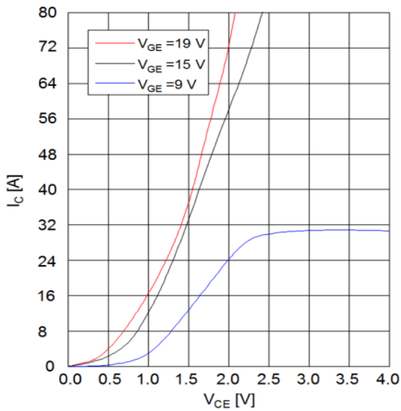
Fig. 1 Typical IGBT Output Characteristics at T_J=25^\circ\text{C}
